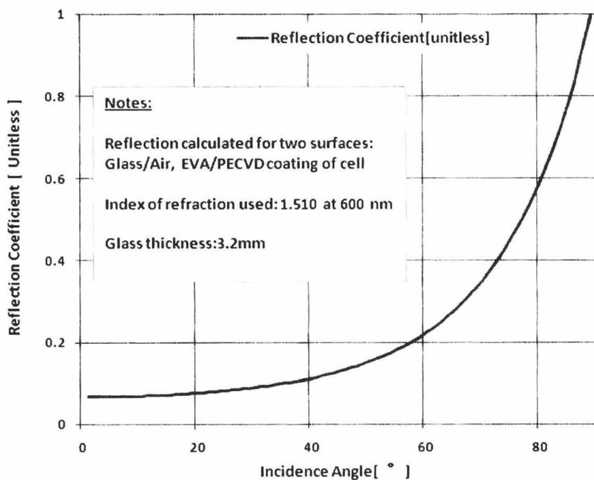
Fig 1 Reflection versus Angle of Incidence
